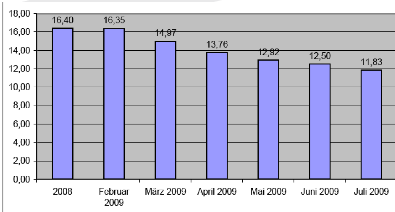
Monthly consumption (kWh/d) FOSTAC MAXIMUS ® M100W installed on 19.02.2009
